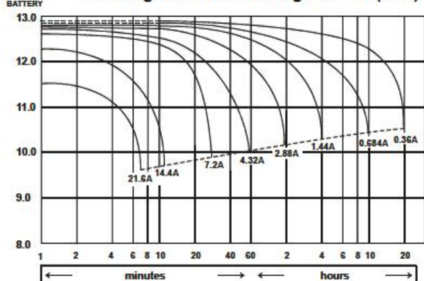
Discharge Time VS. Discharge Current (20°C)
